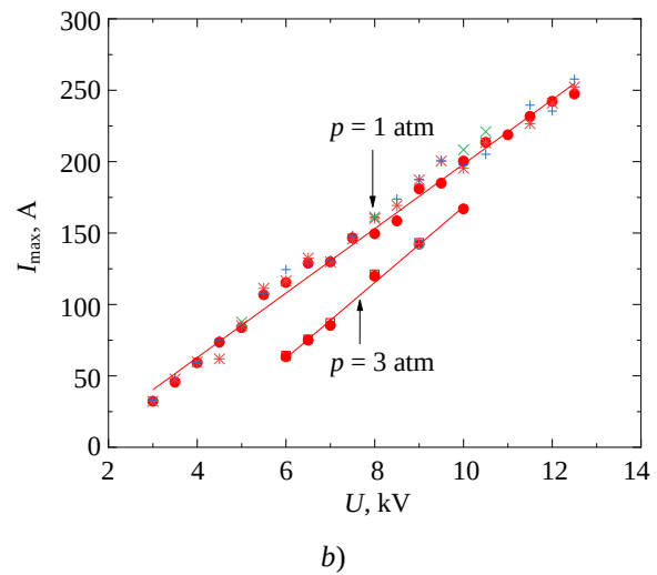
Fig. 3. Amplitude values of the discharge current in the aperiodic mode in various experiment conditions: a) R_b = 2 \Omega , p = 1 \text{ atm} , b) R_b = 52 \Omega , p = 1 \text{ atm} and 3 \text{ atm} .
