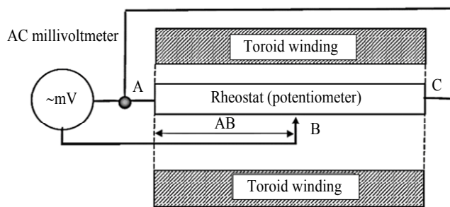
Fig. 2. Schematic of the experiment with a rheostat
