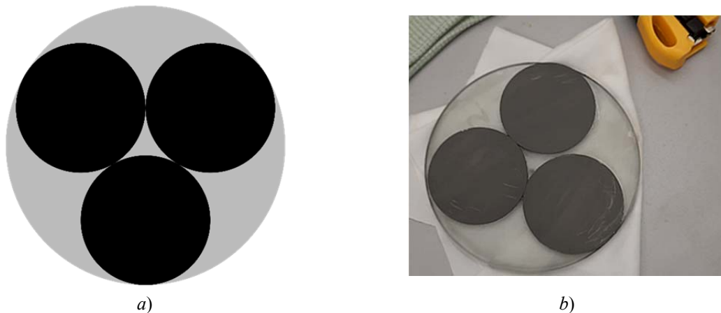
Fig. 2. Illustration of the solution of the two-dimensional packing problem for a disk carrier with a diameter of 112 mm and InSb wafers with a diameter of 50.8 mm (a) and a photo of the InSb wafers bonded to the disk carrier (b)
